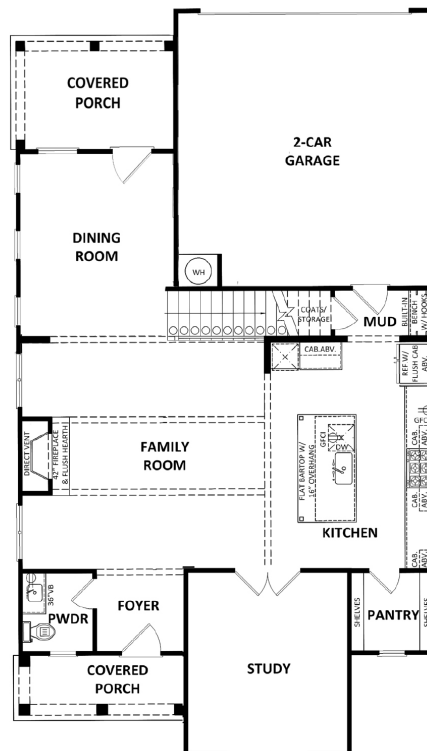
First Floor Plan With Optional Study
